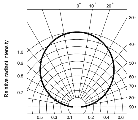
Fig.6 Radiation diagram
